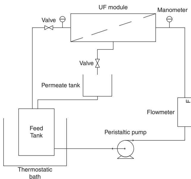
Fig. 1. Scheme of the UF laboratory plant.
