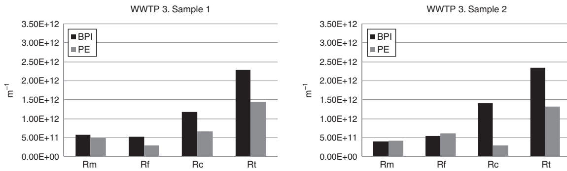
Fig. 4. Comparison between the membrane resistances for the BPI and PE samples from WWTP 3.
