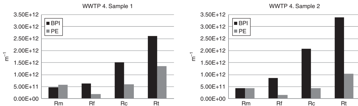
Fig. 5. Comparison between the membrane resistances for the BPI and PE samples from WWTP 4.
