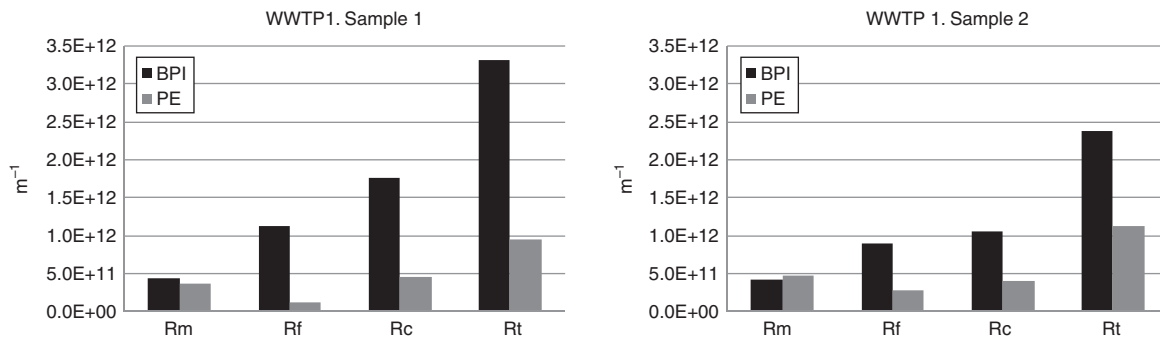
Fig. 2. Comparison between the membrane resistances for the BPI and PE samples from WWTP 1.
