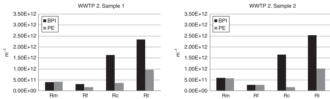
Fig. 3. Comparison between the membrane resistances for the BPI and PE samples from WWTP 2.
